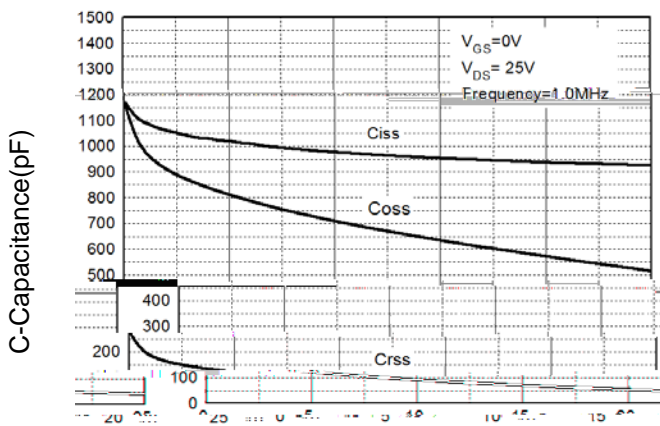
Figure 9: Capacitance Characteristics
